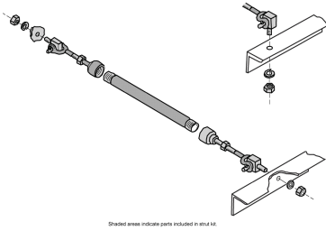
Side Strut Kit for 15 ft microwave antennas
