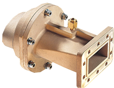
Fixed-tuned PDR40 for elliptical waveguide 37
