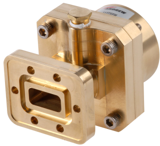
Fixed-tuned PDR120 for elliptical waveguide 127
