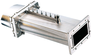
Tunable CPR430G for elliptical waveguide 17
