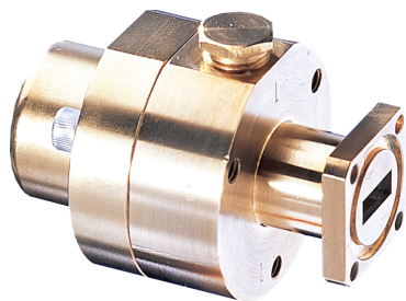
Fixed-tuned PBR220 for elliptical waveguide 240
