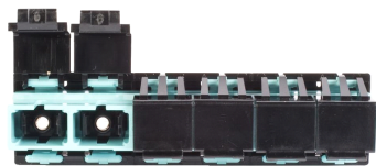
LazrSPEED® SC Multiport Shuttered Adapter, Aqua, Single Pack
