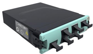
G2 4x6 Multimode OM4 Conversion Module, 6 MPO male ports
