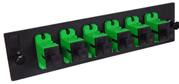
Fiber Optic Adapter Pack, singlemode, 6 simplex ports, SC/APC, green
