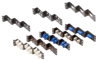
Fiber Optic Adapter Pack Kit, LKH, 12 ST simplex
