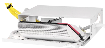
FIST-GSS2 Fiber Splice Panel, 3RU, 19 in, gray
