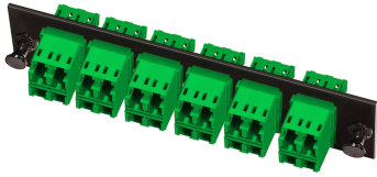
Fiber Optic Adapter Pack Assembly,SM/MM, 12 LC duplex secure, green
