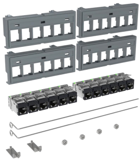
SYSTIMAX 360™ 1100 Evolve SDDM for 6A SL incl jacks and ground kit (4pcs), Gray
