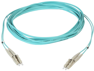
Fiber Optic Patch Cord, Duplex, Multimode, LC/UPC to LC/UPC, aqua, 16 m
