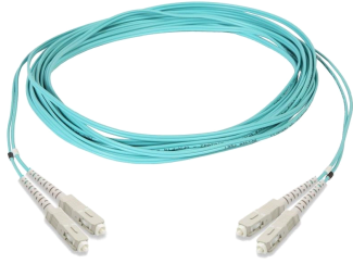
Fiber Optic Patch Cord, Duplex, Multimode, SC/UPC to SC/UPC, aqua, 15 m
