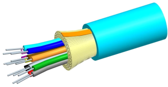
TeraSPEED® Riser Distribution Cable, 4 fiber single-unit
