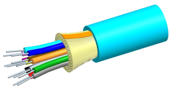
TeraSPEED® Riser Distribution Cable, 8 fiber single-unit
