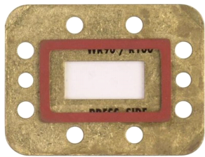
Pressure Window for WR112, 7.05–10.0 GHz, mates to PDR84
