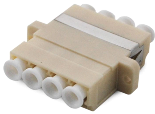
Fiber Optic Adapter, panel mount, LC quad, multimode, beige
