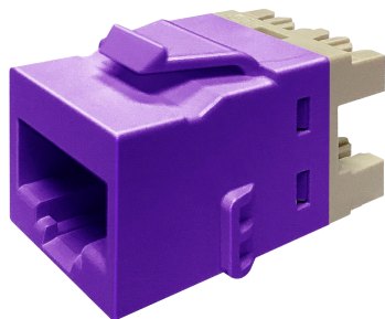
KJ Series Keystone Modular Jack, 8-position, category 6, violet
