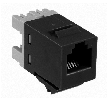
SL110 Series Modular Jack, 8-position, RJ11, category 3, unshielded, without dust cover, black
