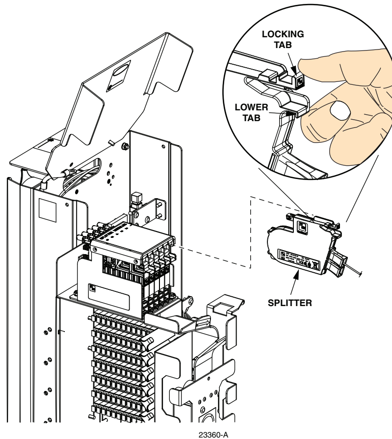
Figure 21. Splitter Installation
