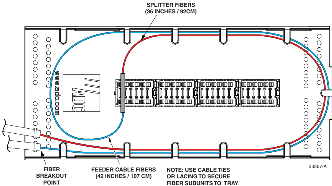
Figure 9. Ribbon Fiber Splice Tray - Feeder Cable Splicing
