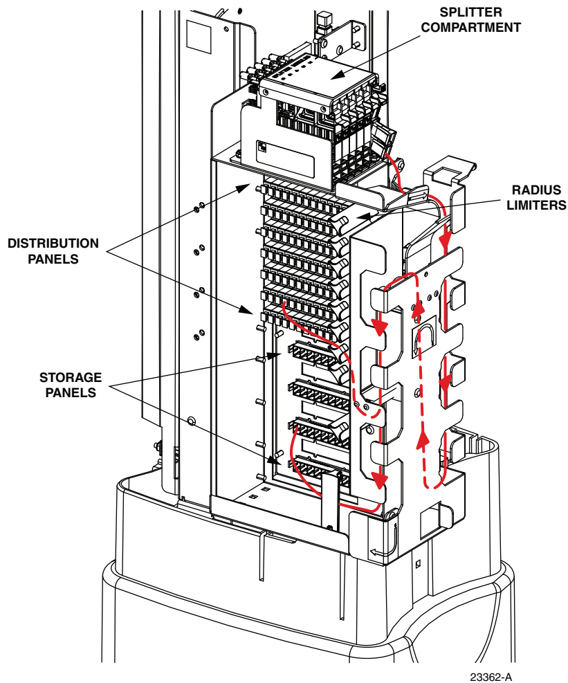
Figure 22. Routing Splitter Output Fibers
