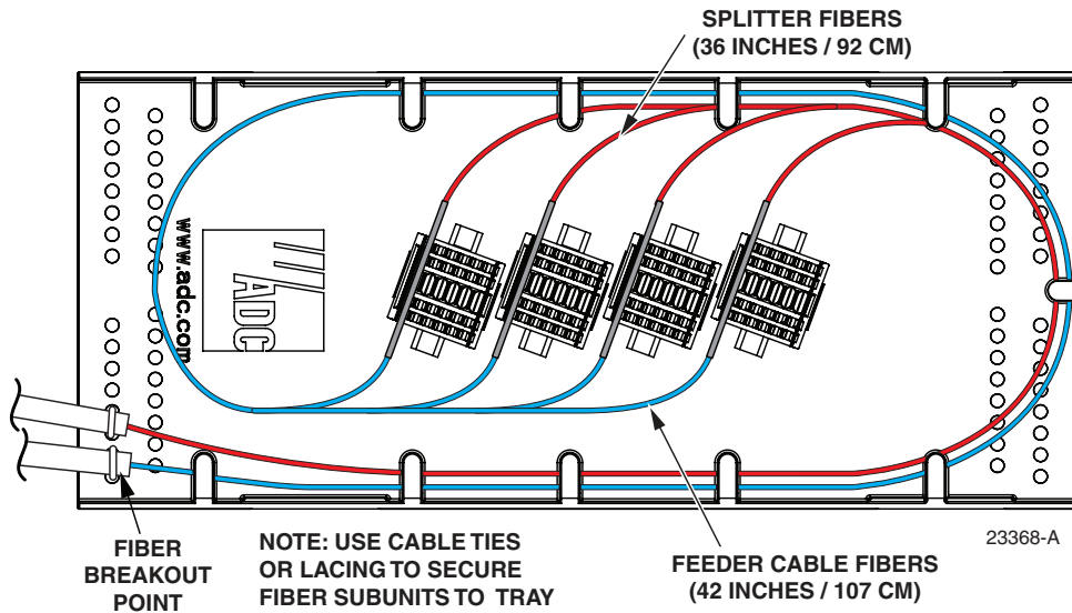
Figure 10. Stranded Fiber Splice Tray - Feeder Cable splicing (Four shown for clarity.)
