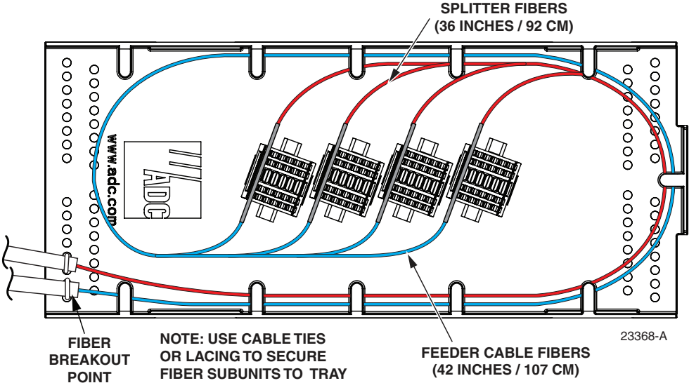
Figure 17. Stranded Fiber Splice Tray - Distribution Cable splicing (Four shown for clarity.)
