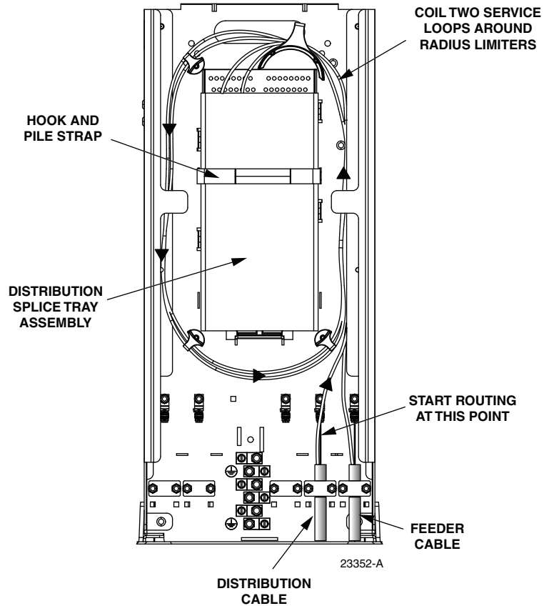
Figure 18. Distribution Splice Tray Installation
