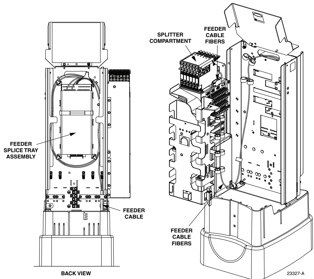
Figure 7. Feeder Splice Tray and Feeder/Splitter Fiber Routing
