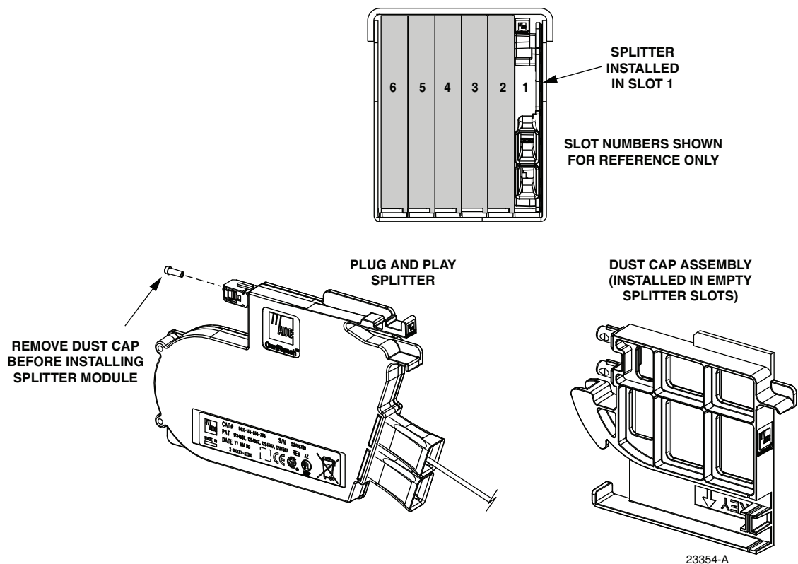
Figure 19. Splitter Module Installation
