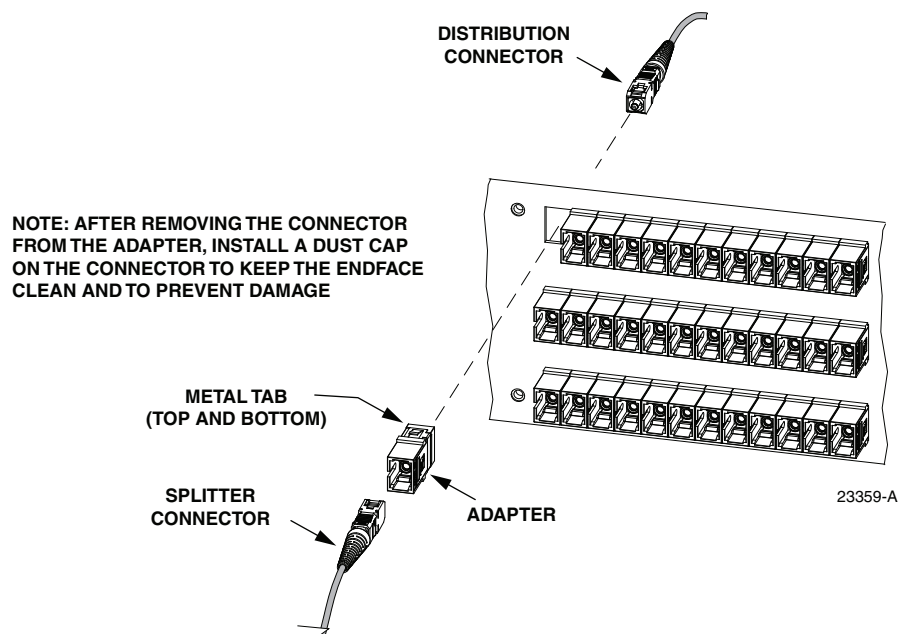
Figure 28. Adapter Removal and Replacement - Typical Distribution Panel
