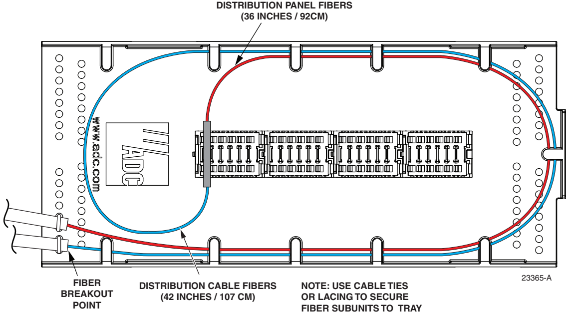
Figure 16. Ribbon Fiber Splice Tray - Distribution Cable Splicing
