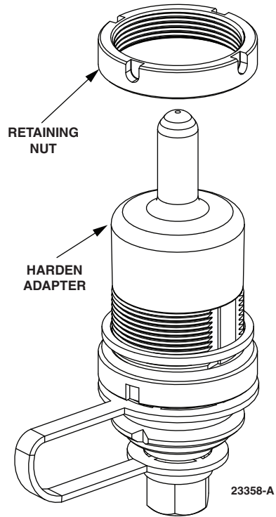
Figure 27. Preparing hardened Adapter
