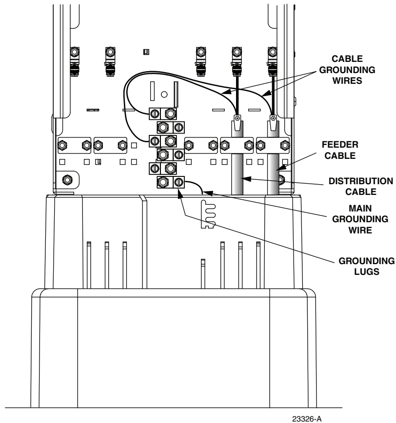
Figure 6. Location of Cable Grounding Lugs
