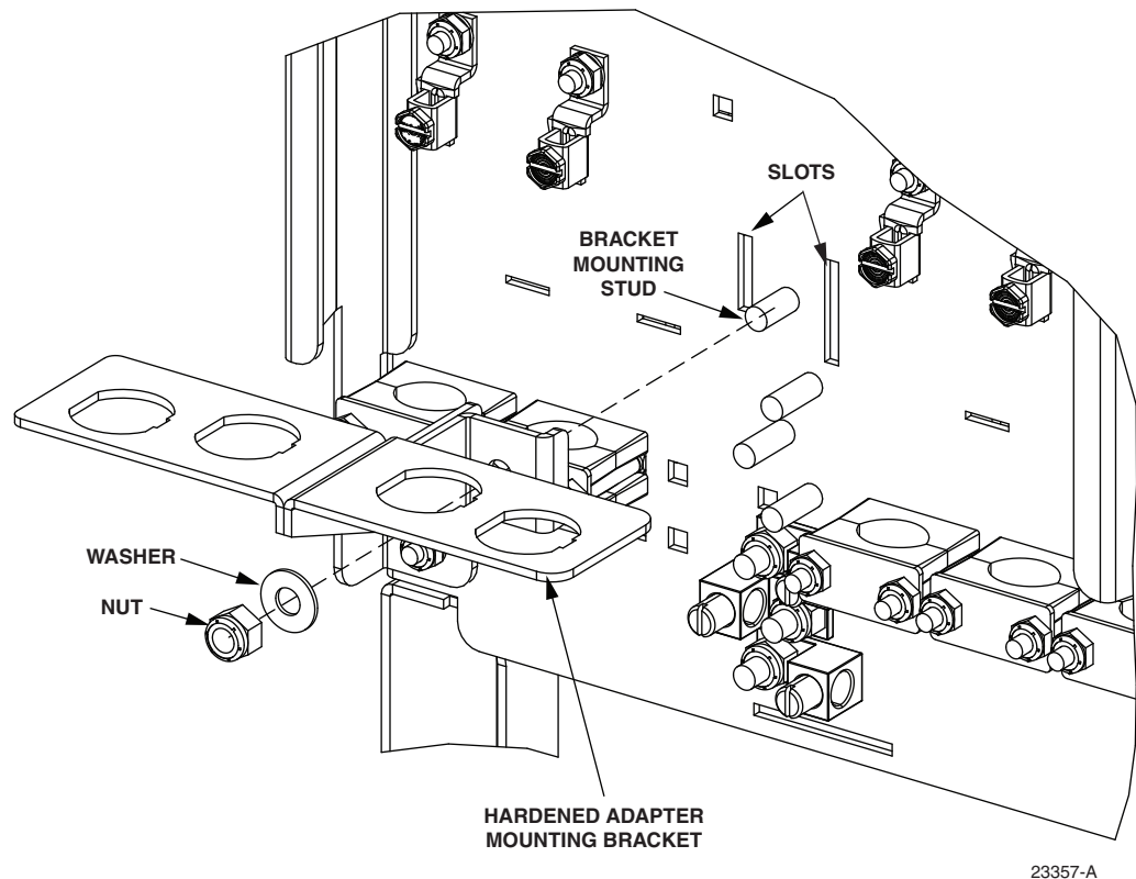
Figure 26. Adapter Mounting Bracket Installation
