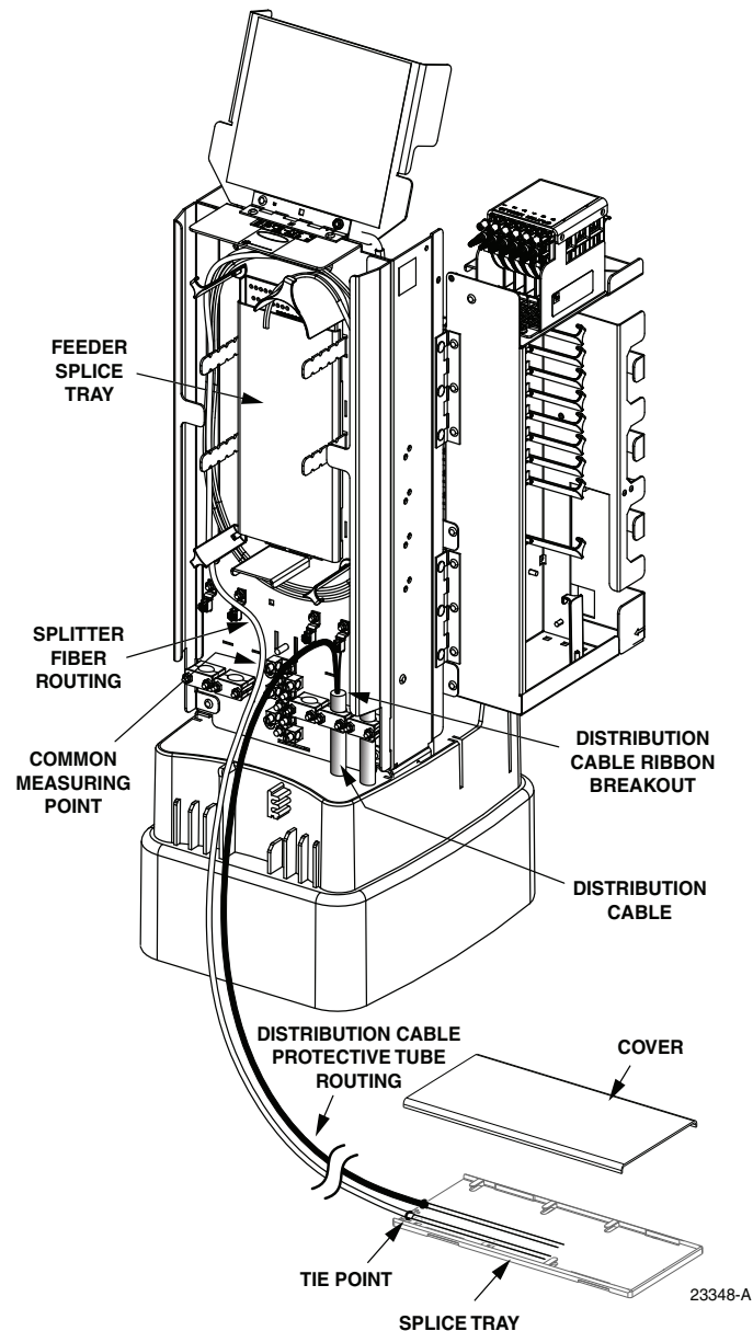
Figure 15. Distribution Fiber Routing
