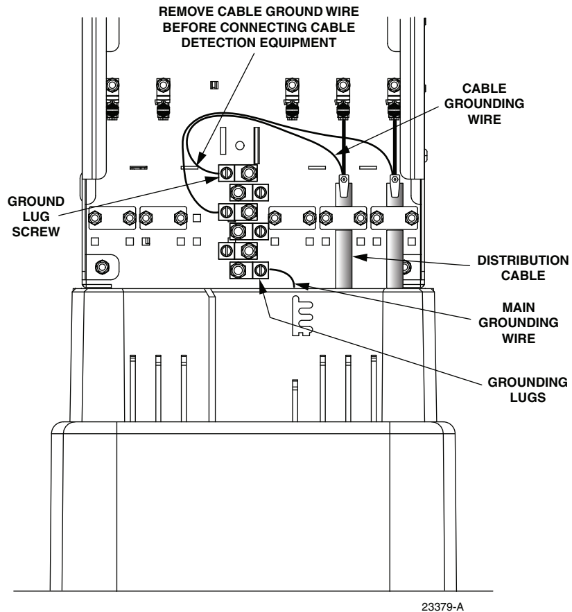
Figure 30. Grounding Block Access
