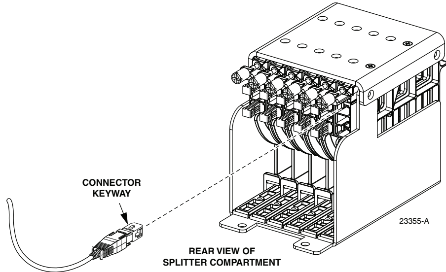
Figure 20. Feeder Cable Connector
