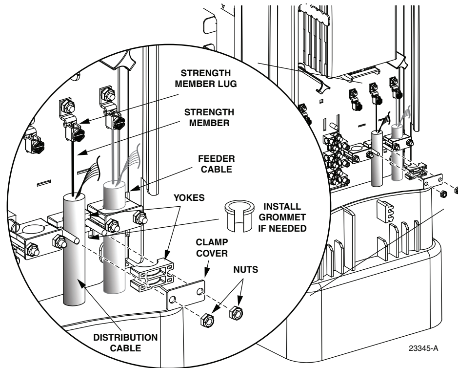
Figure 13. Assembling Distribution Cable Clamp
