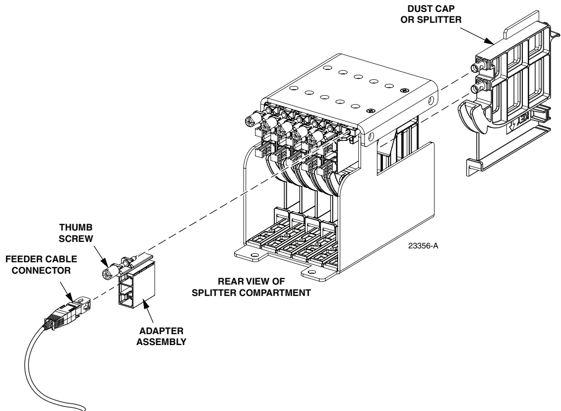
Figure 29. Splitter Compartment Adapter Replacement
