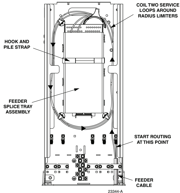
Figure 11. Feeder Splice Tray Replacement
