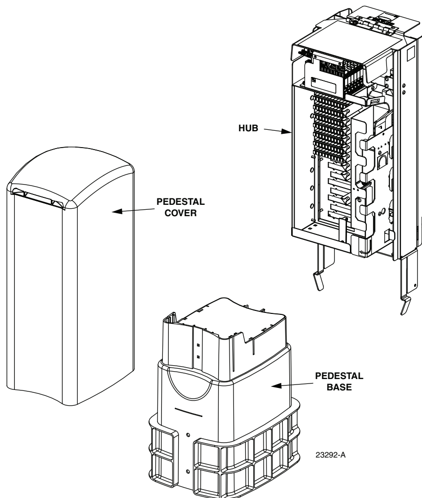
Figure 1. Typical Hub In Pedestal FDH
