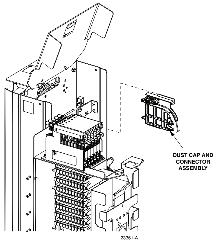
Figure 24. Inserting Dust Cap Assembly Into Splitter Compartment
