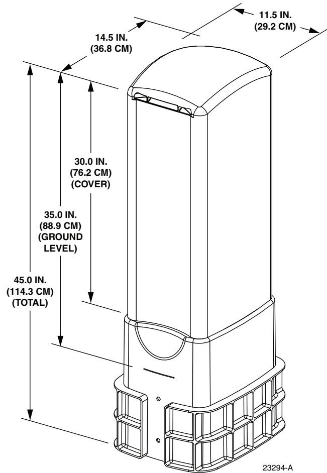
Figure 2. Hub in Pedestal FDH Dimensions
