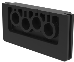
BUDI™ 2S / IFEB10 Branch seal, 4 cables max diameter 7mm - 57 Pieces
