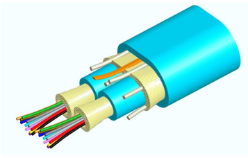
LazrSPEED® Low Smoke Zero Halogen Riser MPO Trunk Cable, 24 fiber with 12 fiber subunits
