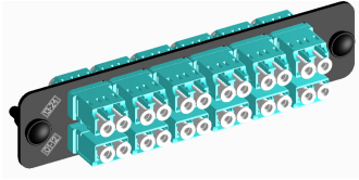
1000-Type Adapter Pack with 12 LC duplex MM adapters, aqua
