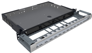
G2 1U Fixed Modular Cassette 4-slot Fiber Panel, unloaded
