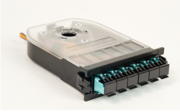
G2 Modular Cassette with 12 LC LazrSPEED® 550 Pigtails
