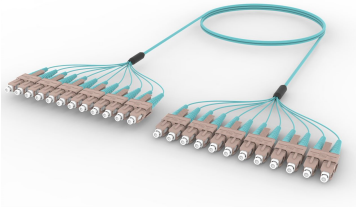
OM3 SC/UPC to SC/UPC 12-Fiber InstaPATCH® 360 Ruggedized Fanout Cable, Low Smoke Zero Halogen
