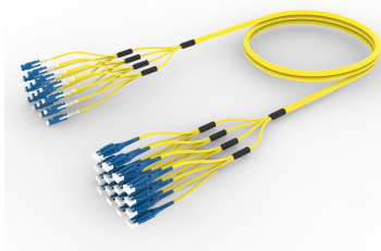
Fiber Optic Patch Cord, Multi-fiber, Singlemode, 24 fibers, SC/UPC to LC/UPC, yellow, 18 m
