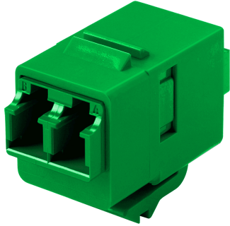
Fiber Optic Insert Adapter, LC, duplex, singlemode/multimode, green
