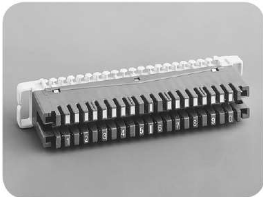
LSA-PLUS Series 2 switching module 10-pair
