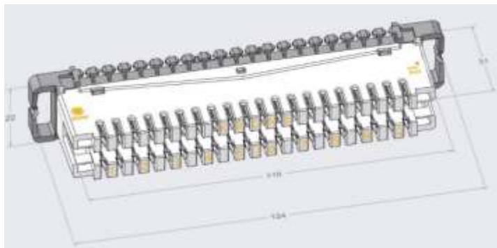
LSA-PLUS Series 2 module 10-pair, basic dimensions in mm.
