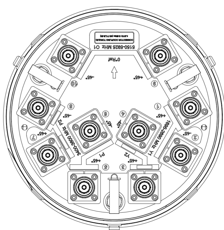
VIEW A-A BRACKET NOT SHOWN
