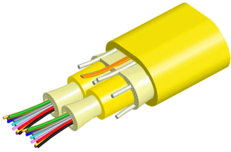
TeraSPEED® Low Smoke Zero Halogen Riser MPO Trunk Cable, 12 fiber subunits
