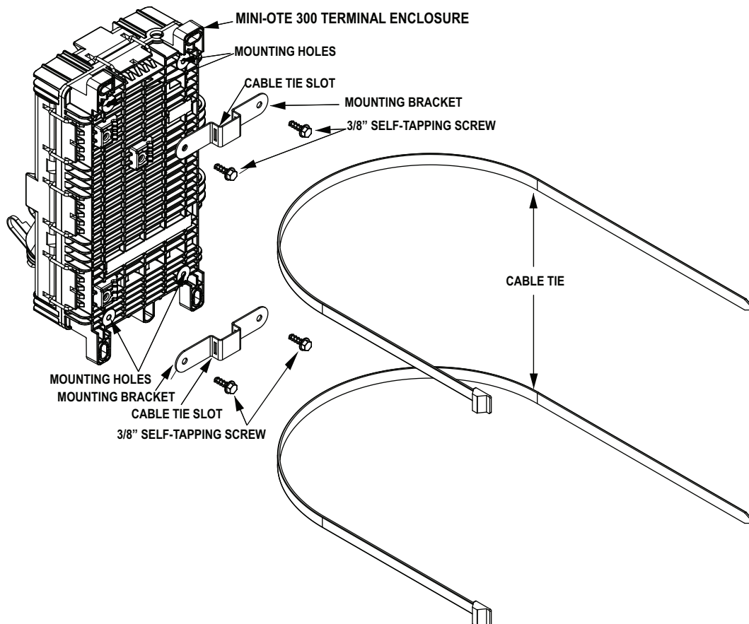
Figure 1. OTE-M Pole-Mount Bracket Kit
