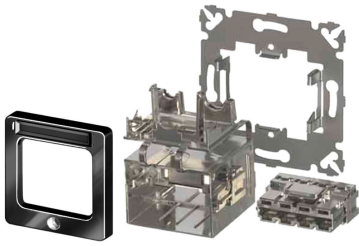
AMP CO Ultra Outlet Installation Kit, shielded, flush mount, DIN 50 x 50, black
