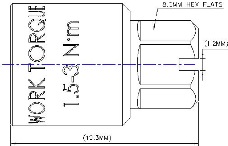
NEX10 FEMALE END CAP ASSEMBLY
