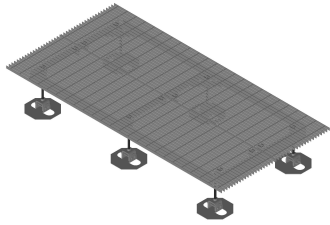
Light Duty Equipment Platform, 4 ft x 8 ft, with six light duty legs
