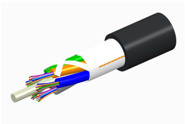
LightScope® ZWP Indoor/Outdoor, Single Jacket All-Dielectric, Low Smoke Zero Halogen (LSZH), Gel-Free, Stranded Loose Tube Cable
