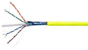
CS44Z1 Cable, category 6A, 4 pair, F/UTP, LSZH, 23 AWG, 1000 ft reel, yellow
