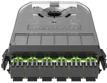
360G2 Cassette 6 SC Angled Singlemode Green with Pigtails A
