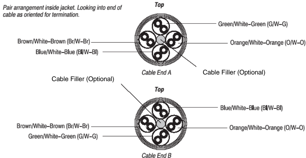
Figure 2. Arrangement of Color-Coded Pairs
