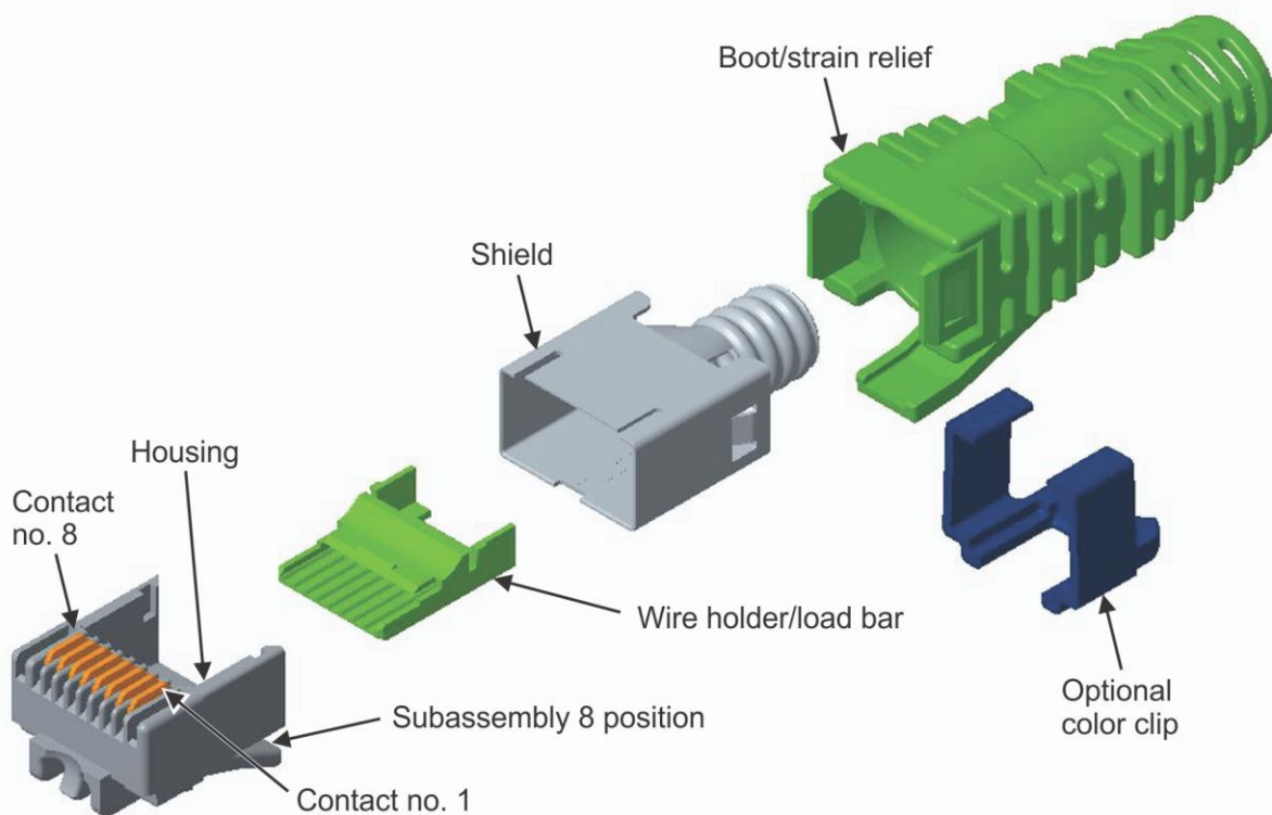
Figure 1. Slim-Line Modular Plug Components
