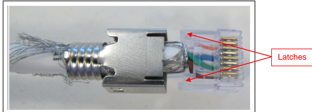
Figure 10. Secure Wire Holder into Housing
