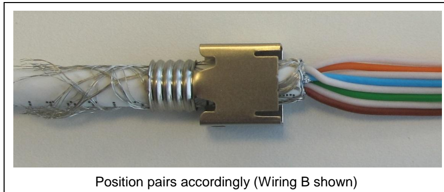
Figure 5. Cable Positioning
