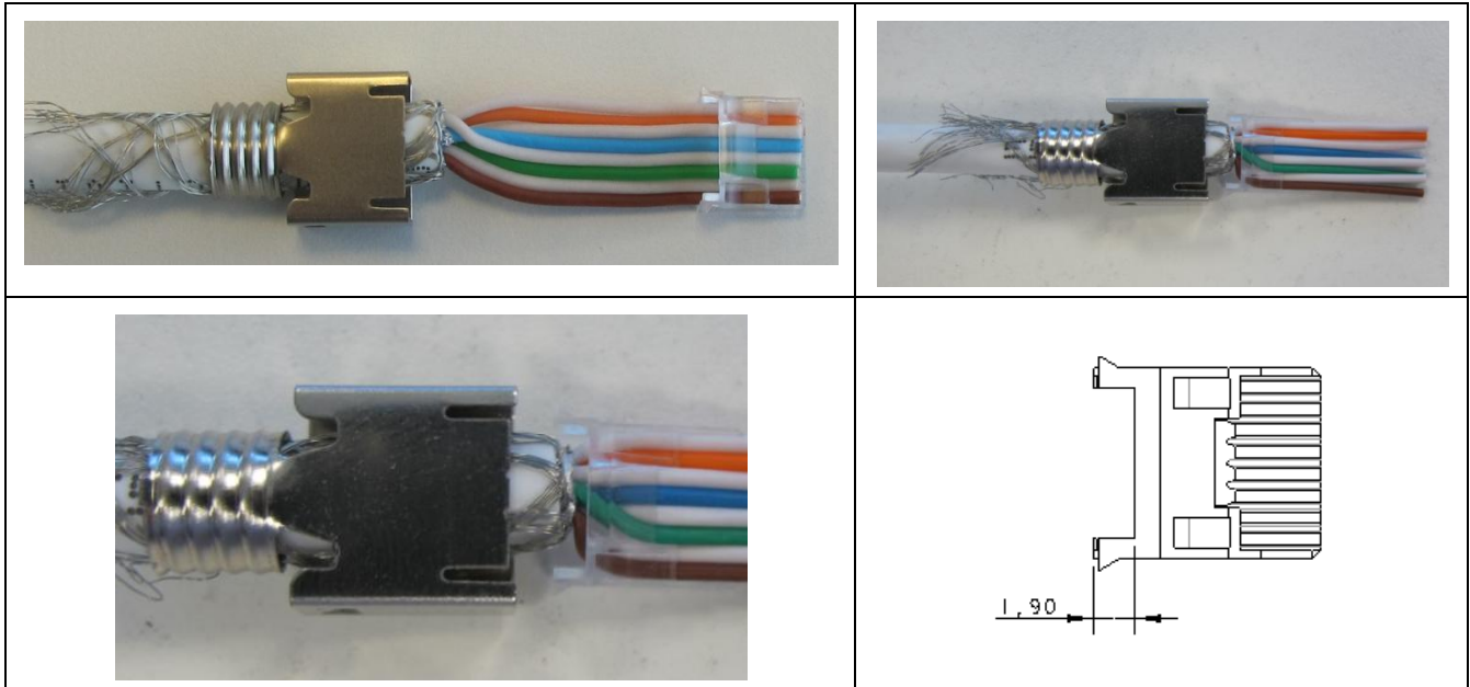
Figure 7. Insert Conductors through Wire Holder
