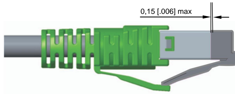
Figure 17. Gap Between Shield and Housing
