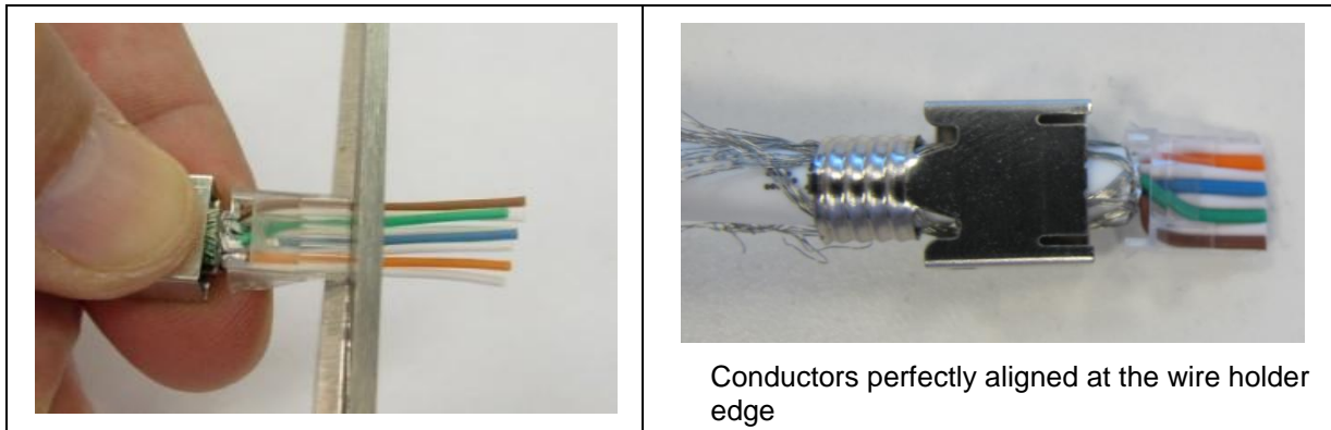
Figure 8. Trim Conductors Even with Wire Holder
