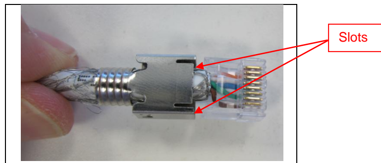
Figure 12. Orient Shield
