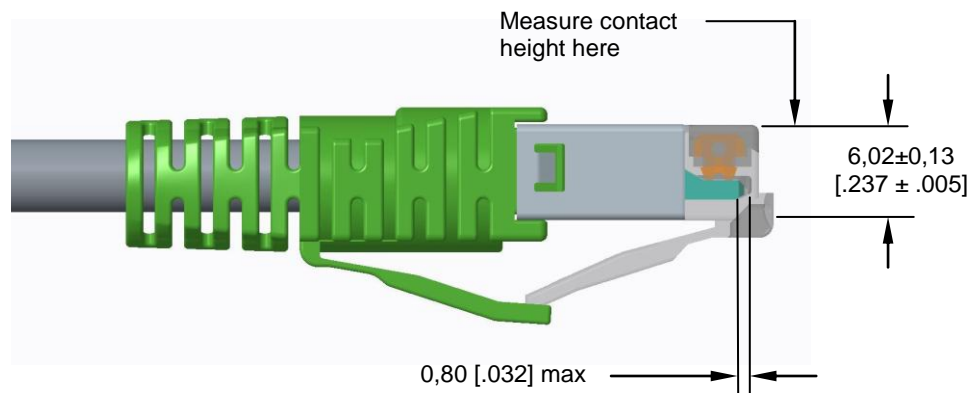
Figure 16. Plug Tolerances
