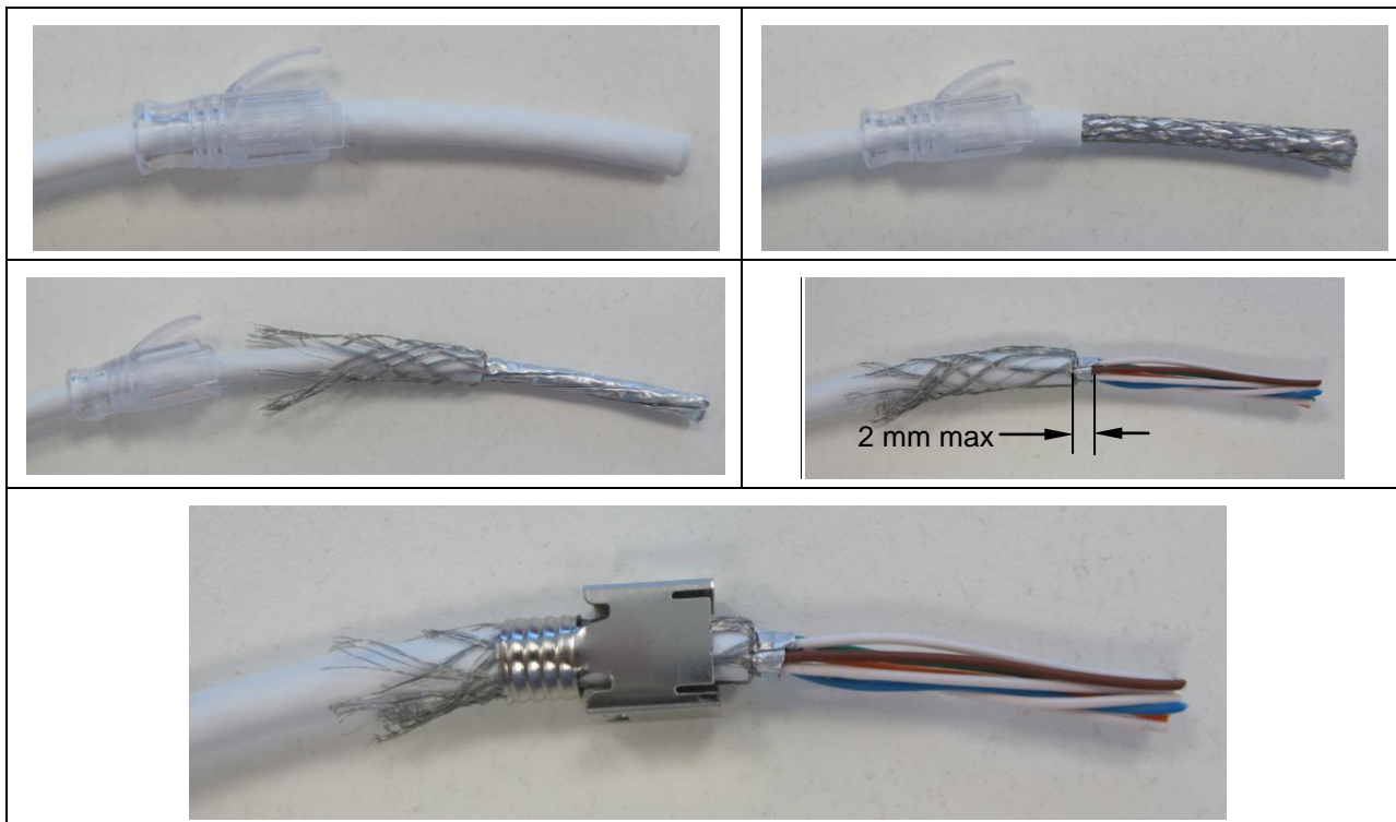
Figure 3: Cable Preparation
