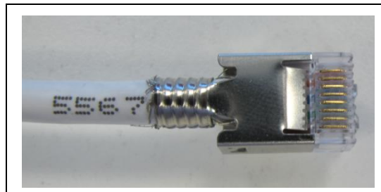
Figure 14. Trim any Braid or Foil
