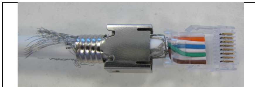
Figure 9. Insert Wire Holder into Plug Housing
