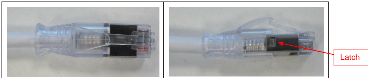
Figure 15. Slide Boot over Crimped Plug
